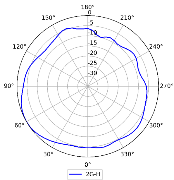
2.4GHz (Horizontal)
