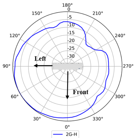
2.4GHz (Horizontal)
