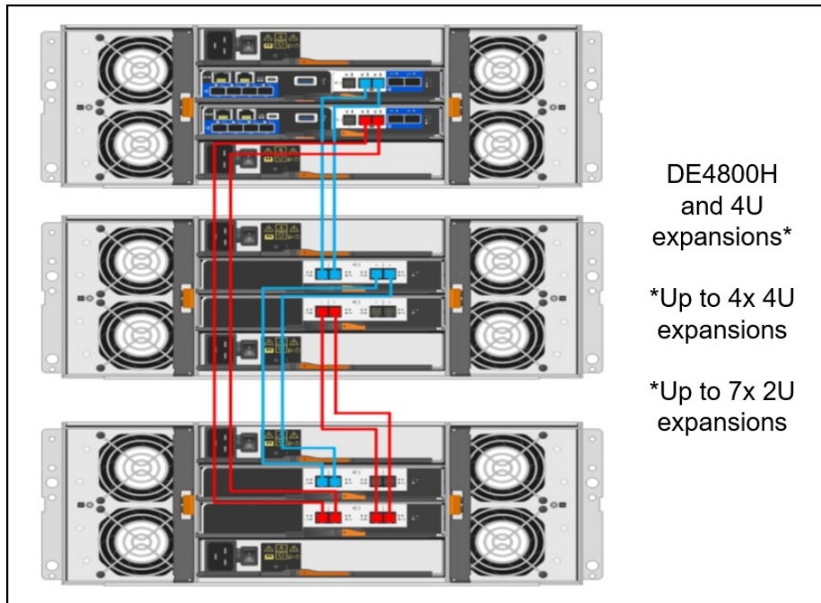
Figure 10. DE4800H 4U60 connectivity topology
