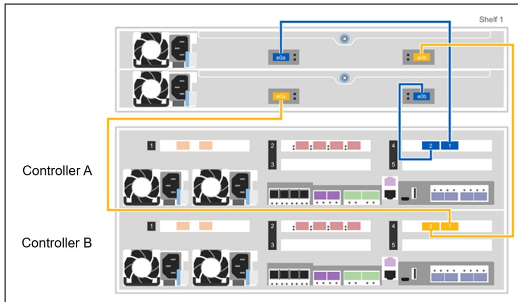
Figure 7. DG7000 NVMe expansion connectivity topology: One enclosure
